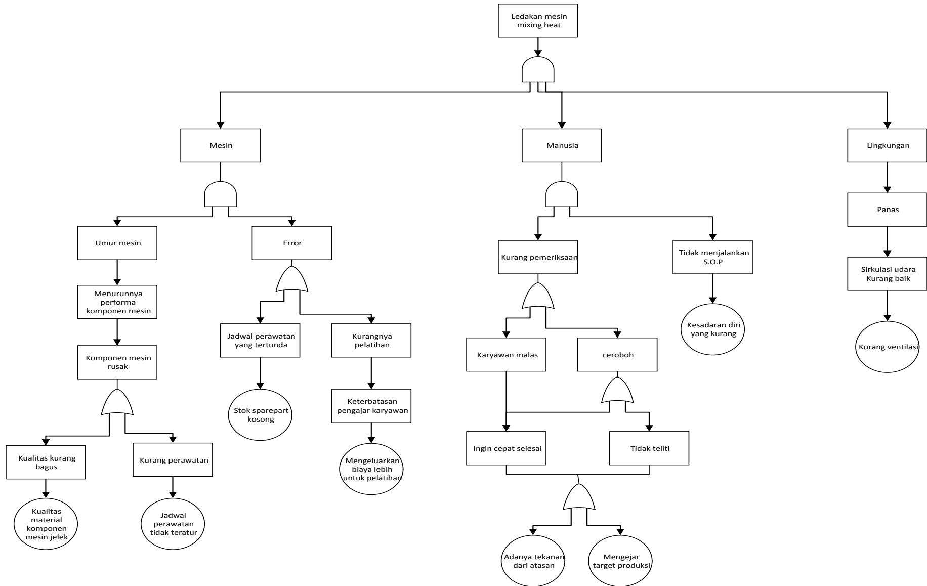
Gambar 4.12 Fault Tree Analysis ledakan mesin mixing heat
